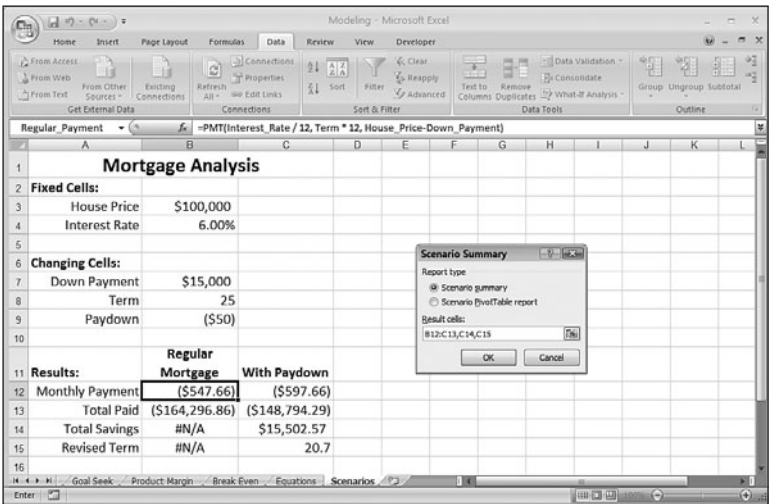
Figure 15.25 Use the Scenario Summary dialog box to select the report type and result cells.
