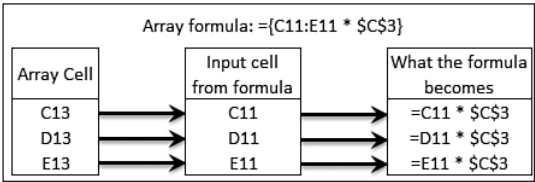
Figure 4.2 When processing an array formula, Excel sets up a correspondence between the array cells and the range used in the formula.
