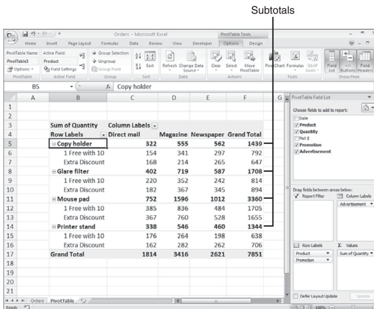
Figure 14.9 When you add multiple fields to the row or column area, Excel displays subtotals for the outer field.
