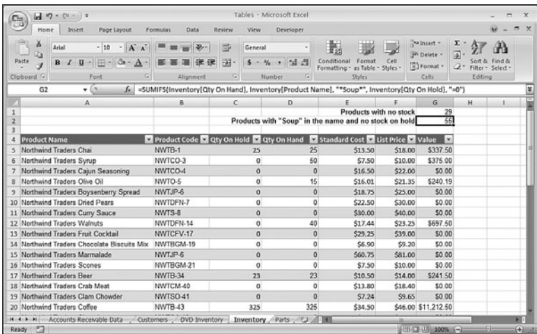
Figure 13.24 Use SUMIFS() to sum the cells that meet one or more criteria.
