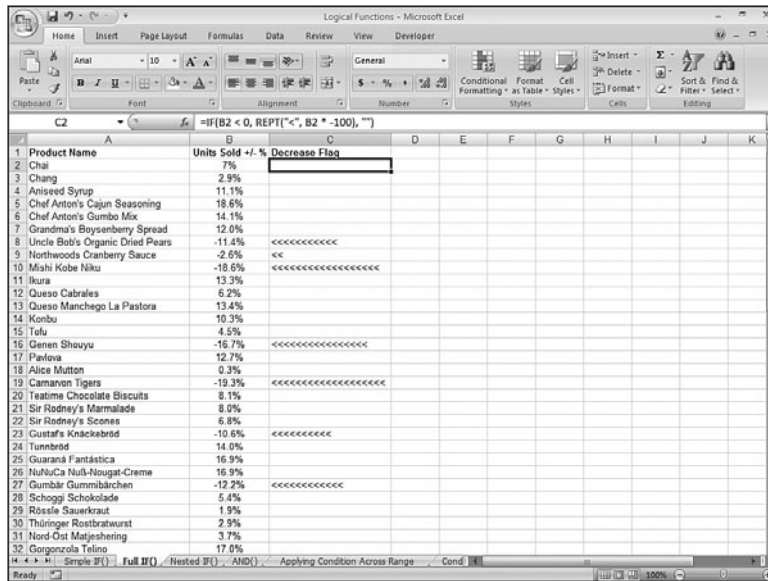
This worksheet uses the full IF ( ) syntax to return no value if the cell being tested contains a non-negative number.
