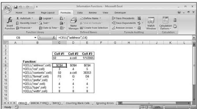
Figure 8.14 Some examples of the CELL() function.
