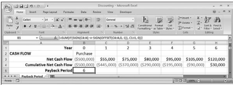
Figure 20.10 Using a formula to calculate the payback period.
