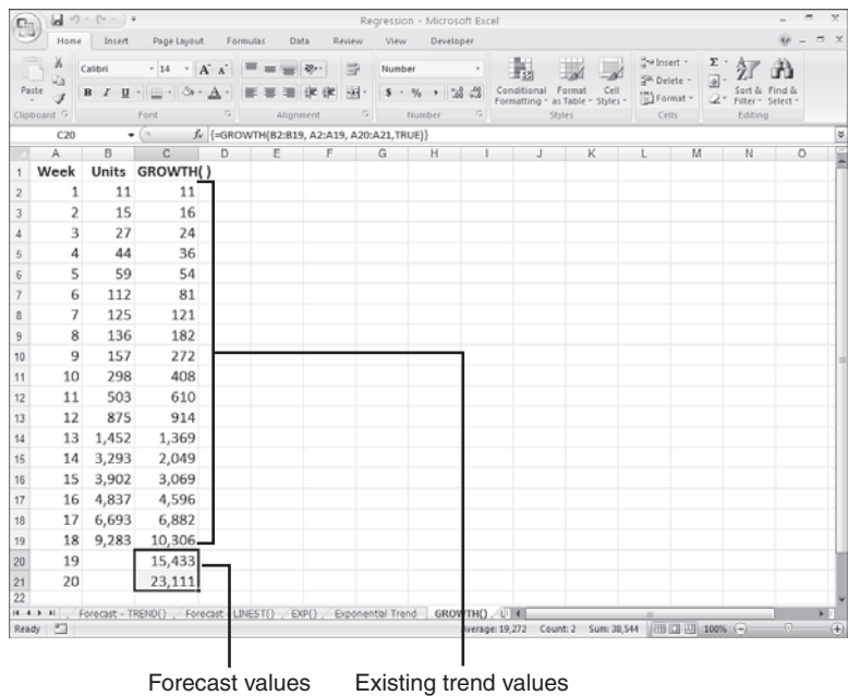
Figure 16.23 The weekly unit sales with existing trend and forecast values calculated by the GROWTH ( ) function.
