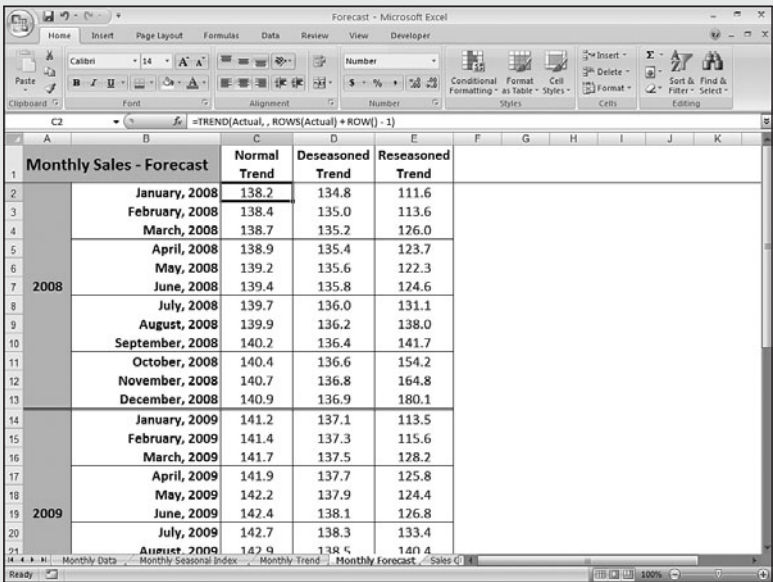
Figure 16.15 The Monthly Forecast worksheet calculates a sales forecast by extending the historical trend data.
