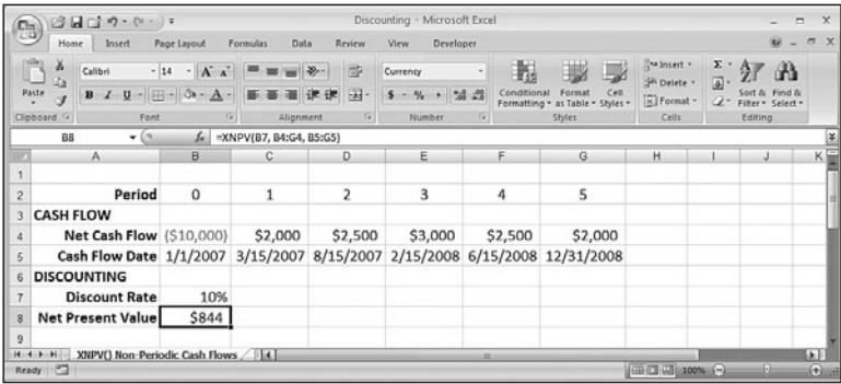
Figure 20.9 Use the XNPV() function to calculate the net present value for a series of nonperiodic cash flows.
