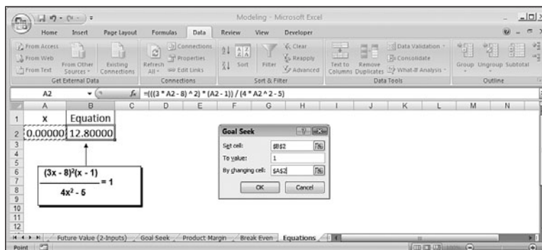
Figure 15.17 Solving an algebraic equation with Goal Seek.
