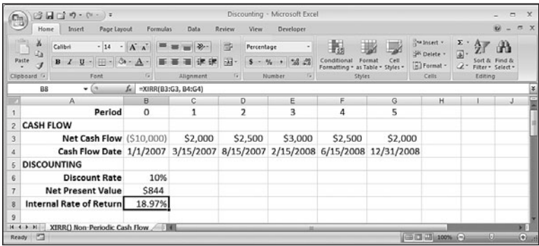
Figure 20.14 Use the XIRR() function to calculate the internal rate of return for a series of nonperiodic cash flows.
