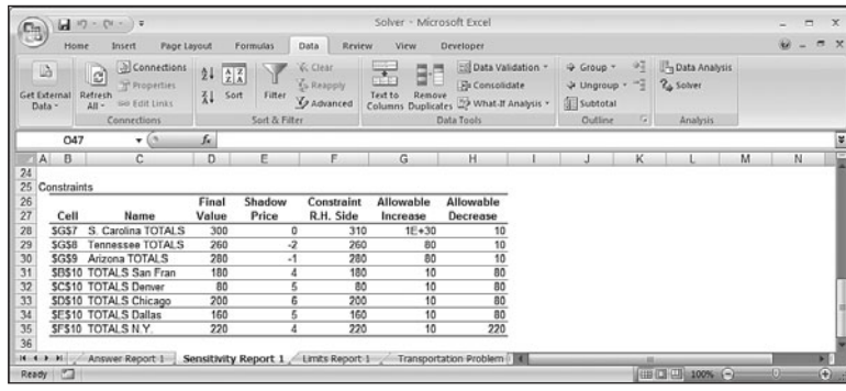
Figure 17.15 The Constraints section of Solver's Sensitivity report.
