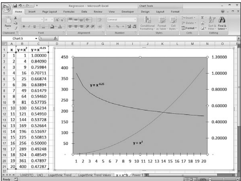
Figure 16.28 Power curves are generated by raising x-values to some power.
