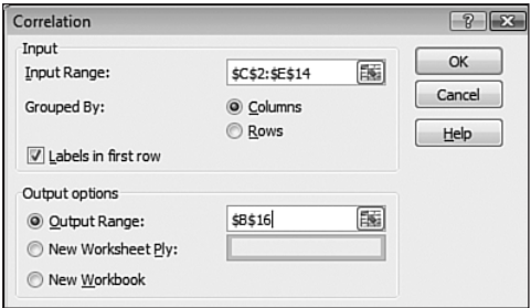
Figure 12.13 Use the Correlation dialog box to set up the correlation analysis.
