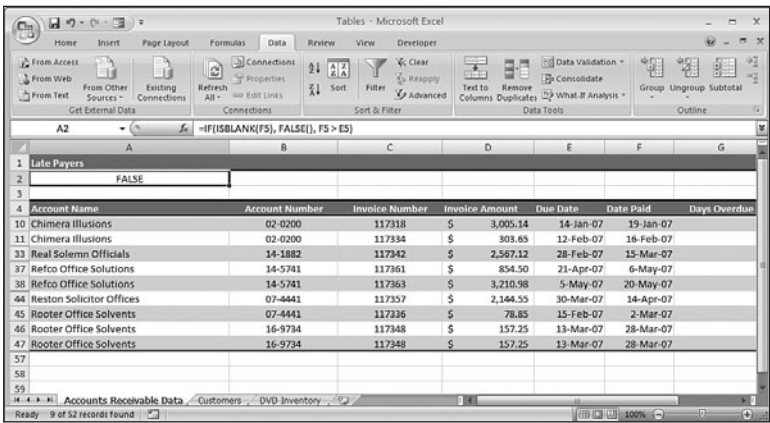
Figure 13.15 Use a separate criteria range column for calculated criteria.
