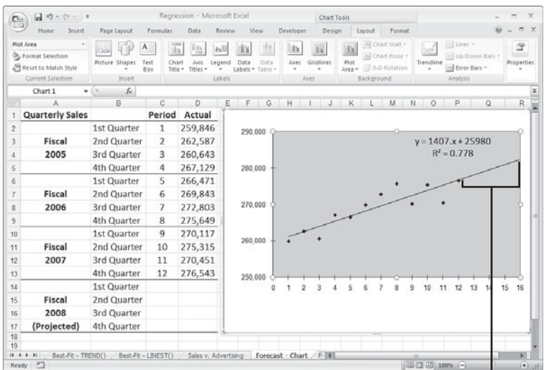
Figure 16.8 The trendline has been extended four quarters into the future.
