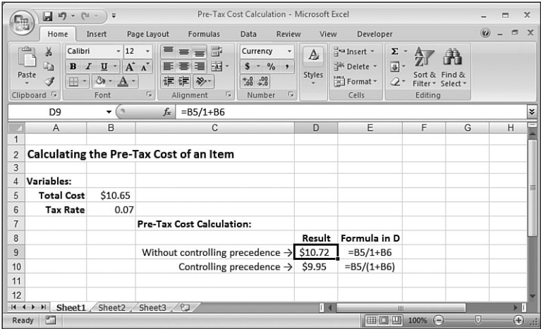
Figure 3.2 Use parentheses to control the order of precedence in your formulas.
