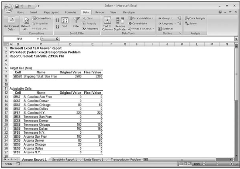
Figure 17.12 The Target Cell and Adjustable Cells sections of Solver's Answer report.
