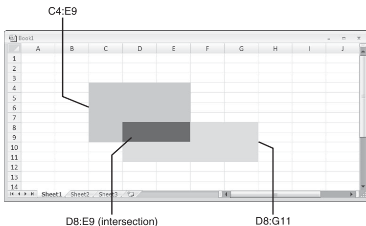
Figure 2.15 The intersection operator returns the intersecting cells of two ranges.
