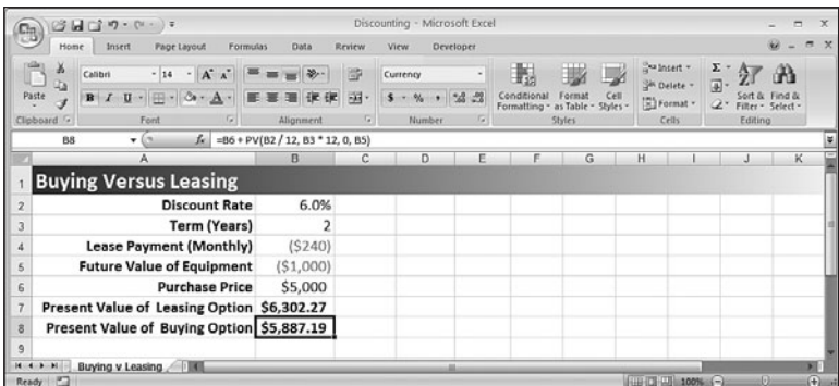
Figure 20.4 Using the PV() function to compare buying versus leasing equipment that has a future market or residual value.
