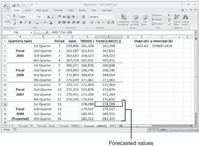
Figure 16.12 The range F14:F17 contains the forecasted values calculated by the regression equation using the slope (H2) and intercept (I2) returned by the LINEST ( ) function.
