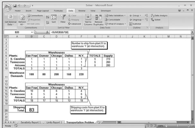
Figure 17.9 A worksheet for solving the transportation problem.
