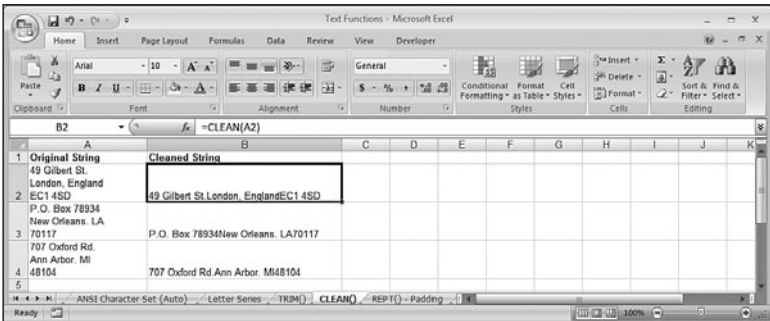
Figure 7.6 Use the CLEAN() function to remove nonprintable characters such as line feeds from a string.
