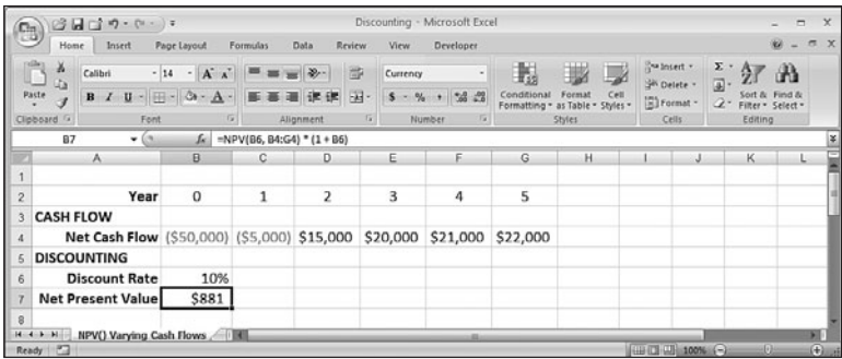
Figure 20.8 To see whether a series of cash flows meets a desired rate of return, use that rate as the discount rate in the NPV() function.
